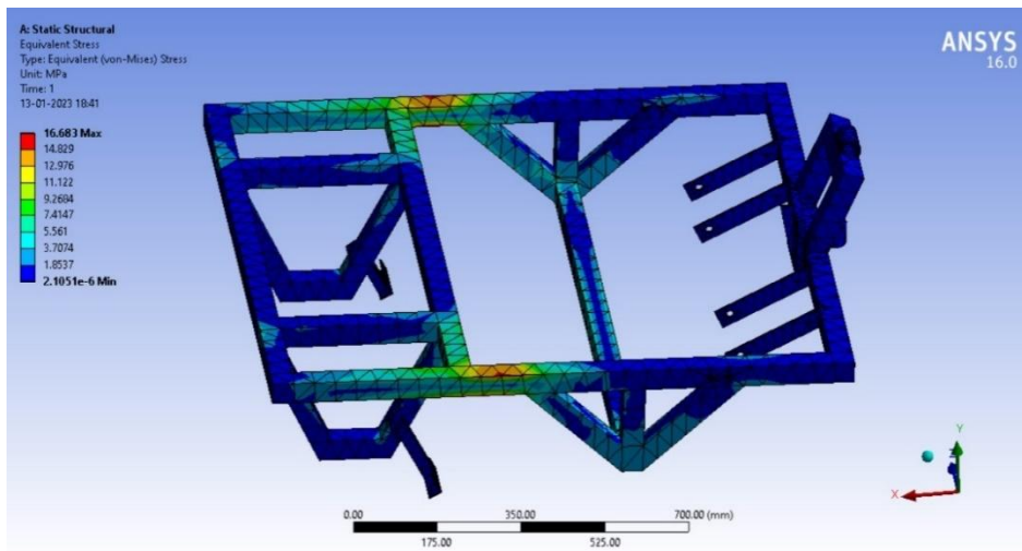
Fig. 5 Equivalent stress
