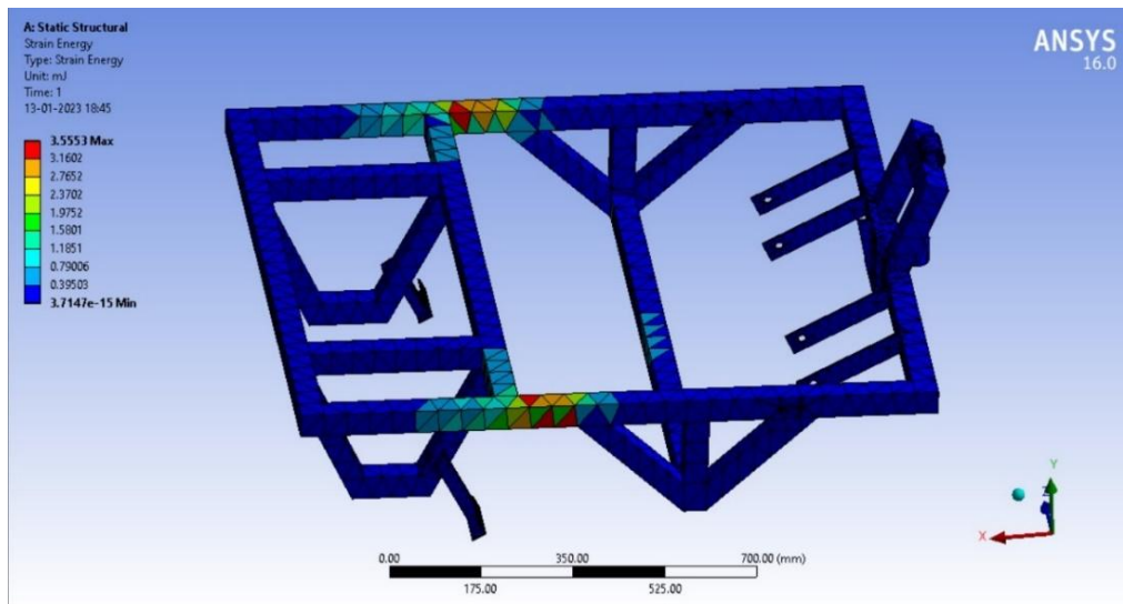
Fig. 8. Strain energy
