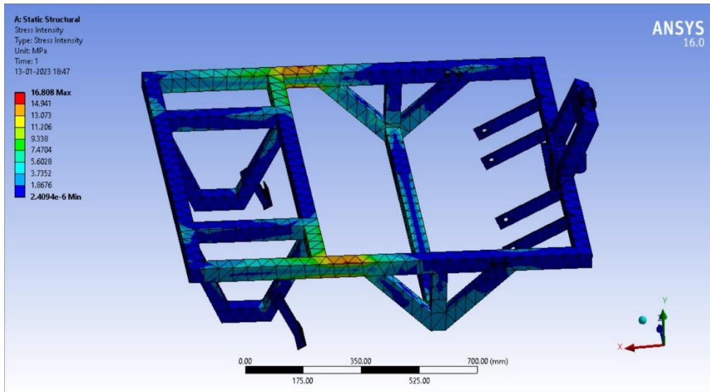
Fig. 7. Stress intensity
