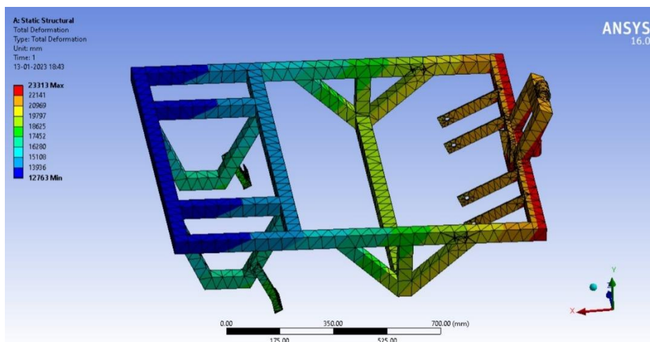
Fig. 3. Total deformation
