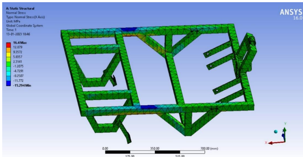
Fig. 6. Normal stress
