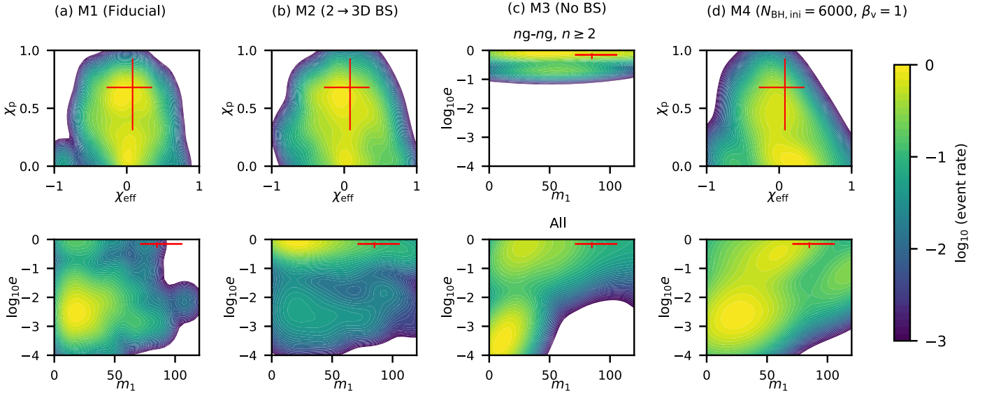
Figure 2. Detection rate distributions of several parameters for the same models as in Figure 1. The top and bottom rows show distributions of \chi_{\text{eff}} - \chi_p and m_1 - \log_{10} e_{10\text{Hz}} , respectively, while in model M3, m_1 - \log_{10} e_{10\text{Hz}} are shown for all mergers (bottom row) and mergers among n -generation ( n \geq 2 ) BHs (top row). The error bars correspond to the 90 percentile credible intervals for GW190521 (Abbott et al. 2020a), while we here roughly assume e_{10\text{Hz}} = 0.7_{-0.2}^{+0.1} , referring to Gayathri et al. (2020).
