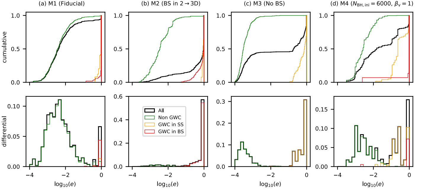
Figure 1. Cumulative (top row) and differential (bottom row) detection rate distributions of the eccentricity at 10 Hz e_{10\text{Hz}} for models M1 (a), M2 (b) in which BS interactions occur in 2 \rightarrow 3D space (Section 2.5), M3 (c) in which BS interaction does not operate, and M4 (d) in which the initial BH number is low ( N_{\text{BH}, \text{ini}} = 6000 , \beta_v = 1 ). In addition to the sum of all binary mergers (black), separate contributions from binaries due to the non-GWC (green), SS-GWC (orange), and BS-GWC (red) are shown.
