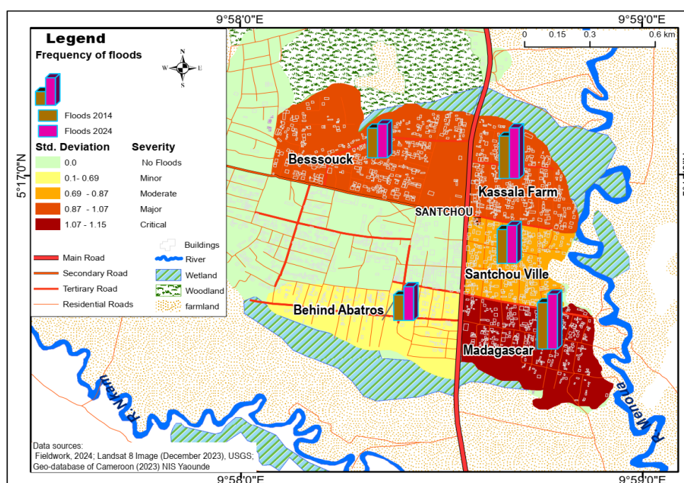
Fig. 3. Spatial variation of flood severity in Santchou
