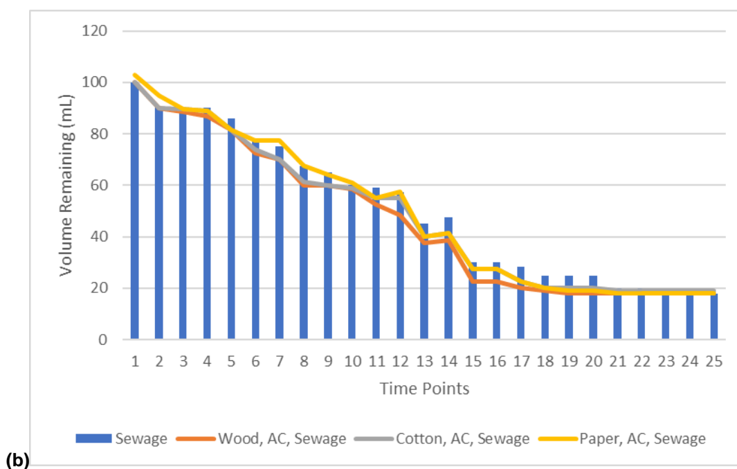
Fig. 6. The solar thermal evaporation test results: (a) acid-treated carbon in seawater, (b) acid-treated carbon in sewage
