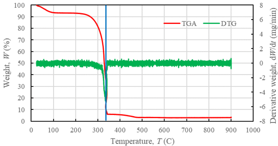
Fig. 5. TGA and DTG of wood in the temperature range from 23 to 900°C
