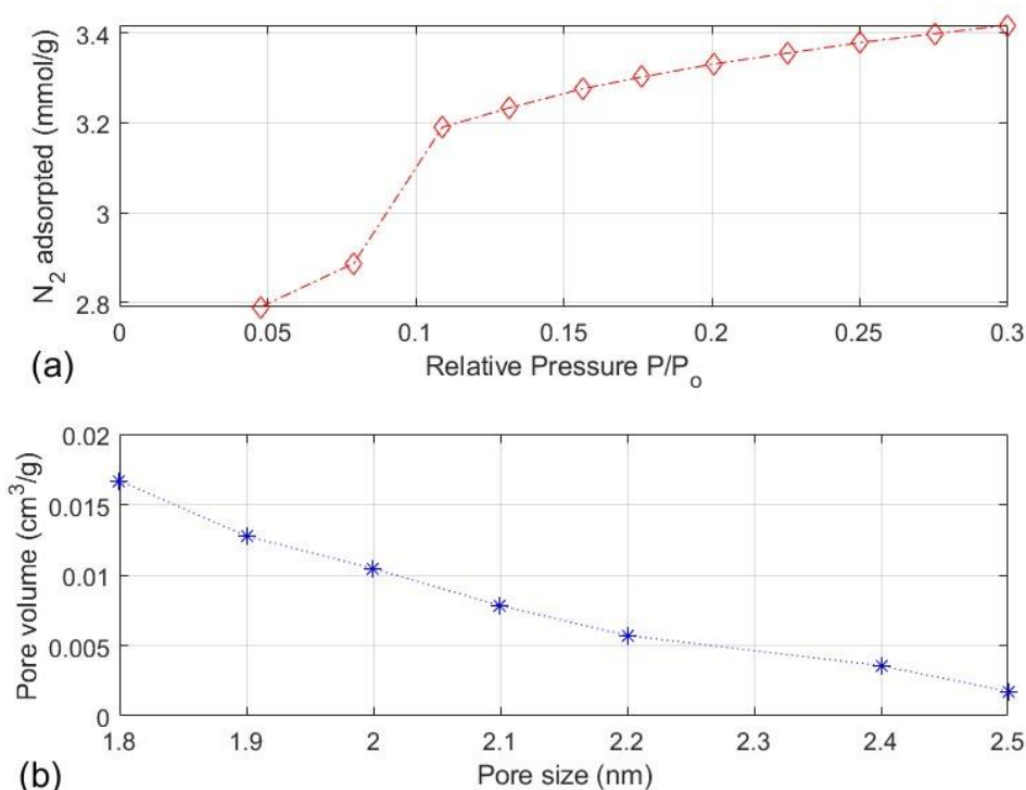
Fig. 10. The BET results for the wood derived carbon: (a) isothermal, (b) pore size distribution
