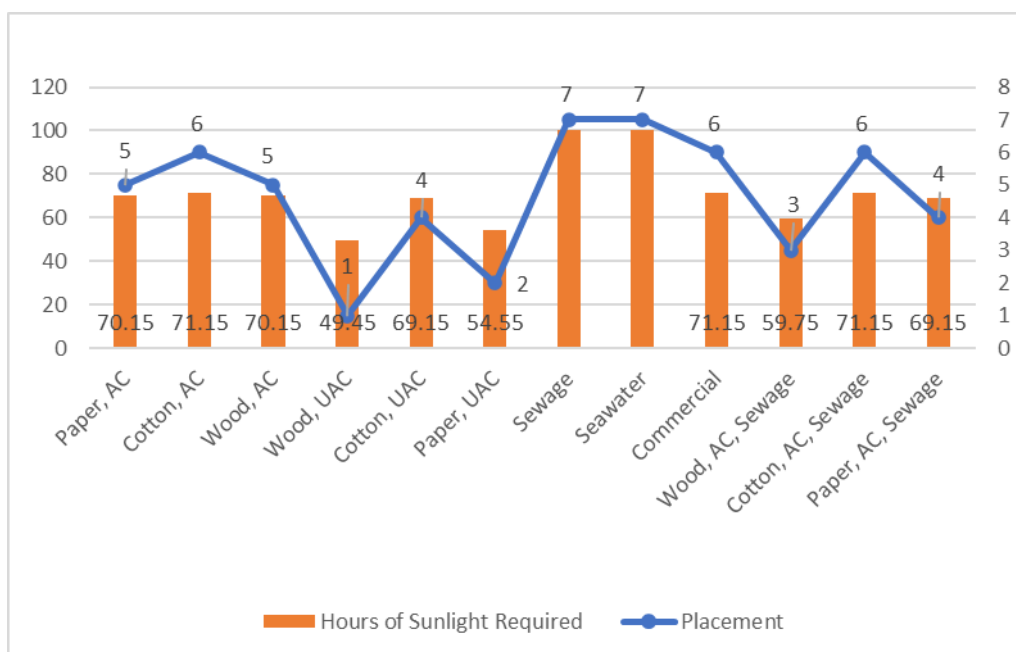
Fig. 7. Hours of sunlight are required to evaporate 100 mL of liquid. (Note: The evaporation hours for the control samples of sewage and seawater without any carbon addition were not recorded)
