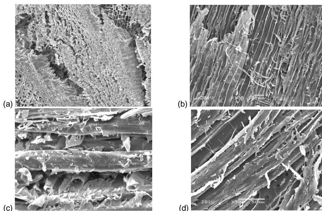
Fig. 4. Scanning electron microscopic images of wood before and after carbonization: (a) transverse cross-section view of wood before carbonization, (b) longitudinal cross-section view of wood before carbonization, (c) higher magnification showing the layered structure of wood before carbonization, (d) the shrinkages and cracking of the ligaments, pore expansion and fibrillation of wood after carbonization
