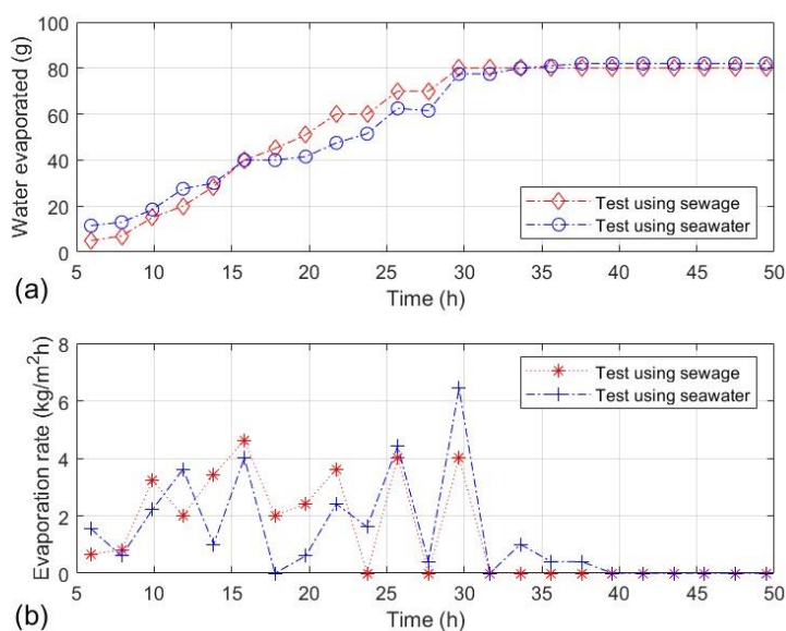
Fig. 8. Solar thermal evaporation performance of the wood derived carbon being tested in sewage water and seawater: (a) accumulative water evaporation amount, (b) water evaporation rate
