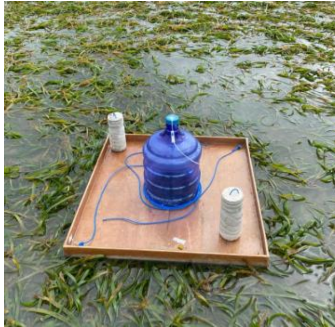
Fig. 2. Operational placement of Rh-Chamber on gas sampling in the seagrass sediment area
