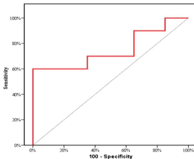
Fig. 3. ROC curve for the angle of rotation of the origin of the aortic to predict pulmonary atresia
