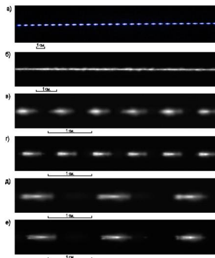
Fig. 5. Time controlled evolution of trains in the space for F=20\text{Hz} , 50\text{cm/s} and for F=25\text{kHz} , 250\text{cm/s} correspondingly
