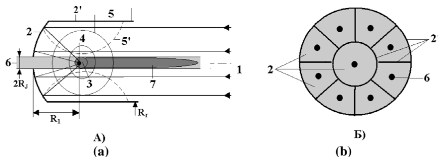
Fig. 3. Scheme of reflector (a) and possible structure of matrix of reflectors (b) for LJE
