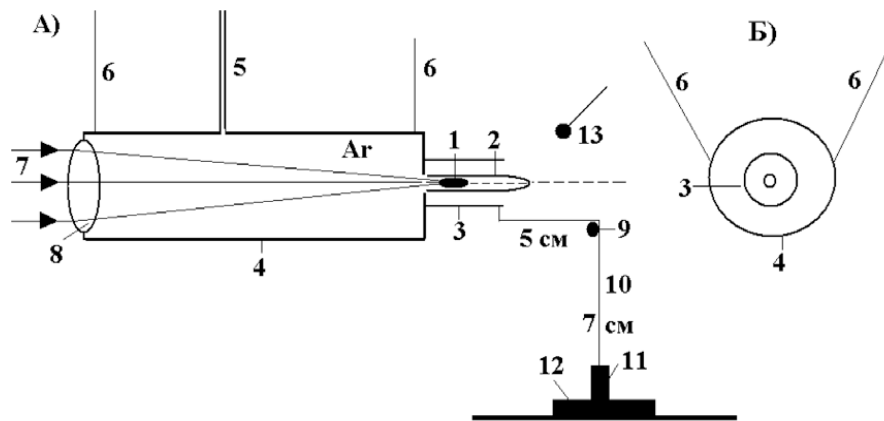
Fig. 4. Scheme of experimental setup
