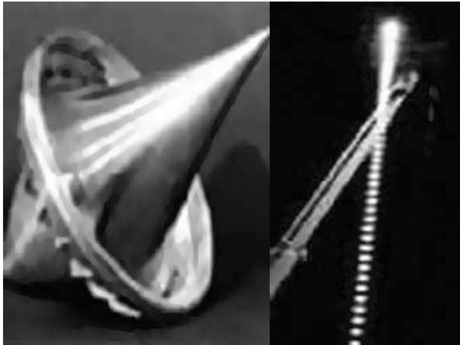
Fig. 6. Launch of vehicle by low rate P-P laser (Rep. rate -20Hz, P=10kW)
