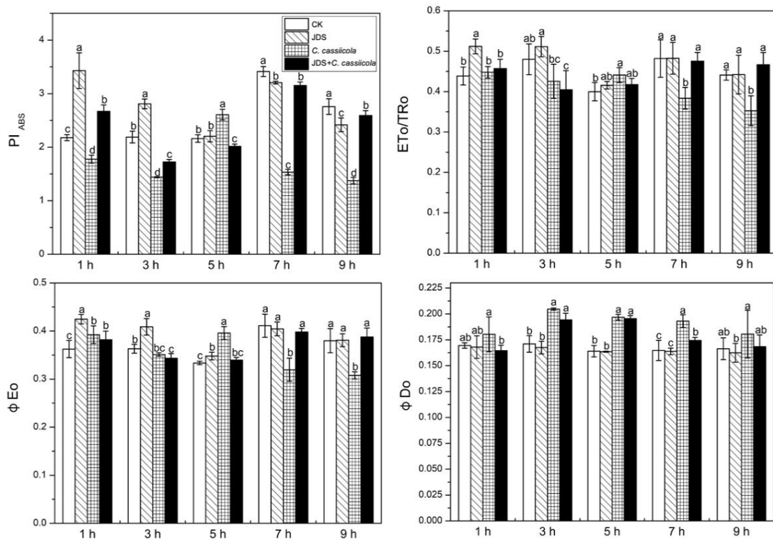
Fig. 2. Effects of JDS on F0, Fm, \phi P , Fv/F0, Dlo/CSO, RC/CSO, TRo/CSO, ET0/CSO, PI ABS , \phi o , \phi Eo and \phi Do under the stress of C. cassiicola
