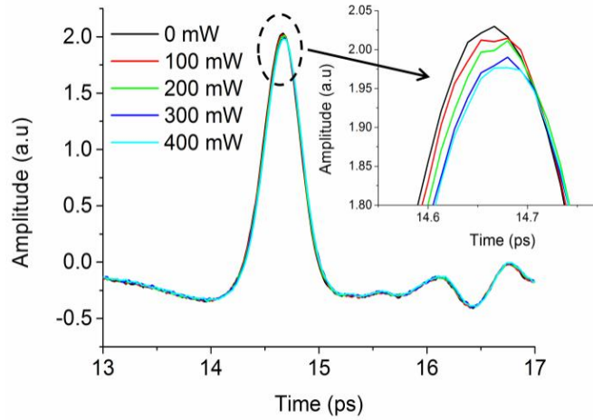
Fig. 6. Waveforms of the THz pulses transmitted through the excited monoSi solar cell at 365 nm with various illumination powers
