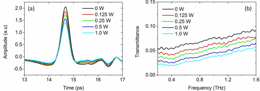
Fig. 3(a). Waveforms of the THz pulses transmitted through the excited monoSi solar cell at 800 nm with various illumination powers. (b) Transmittance obtained from the waveforms in (a)
