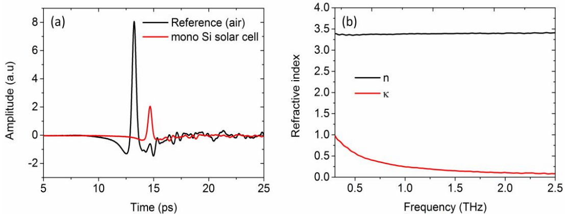
Fig. 2(a). Waveforms of the terahertz pulses of free space and the pulses through mono Si solar cell. (b) Complex refractive index with real part n and imaginary part \kappa of the cell
