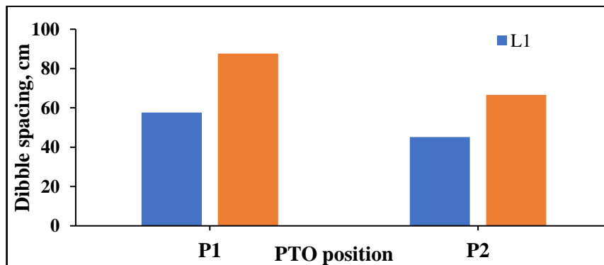
Fig. 4. Effect of gear position and PTO position on dibble spacing ***Figures and tables should be referred to in the body of the paper
