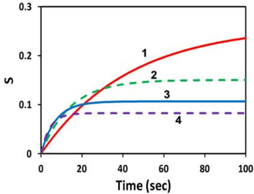
Fig. 6. The S-function profiles for Type-I( S_1 ) (at z=0 ), for intensity I_0= (3,9,18,30) \text{ mW/cm}^2 (curves 1,2,3,4), for C_0=0.1\% and D=500 \text{ um} , based on analytic formula Eq. (8.a)
