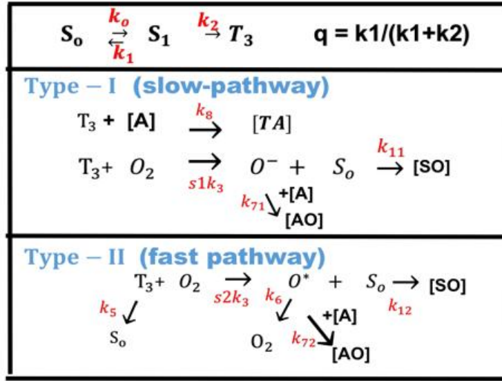
Fig. 3. The kinetics of CXL showing the rate constants associate with Fig. 2 [10,17]
