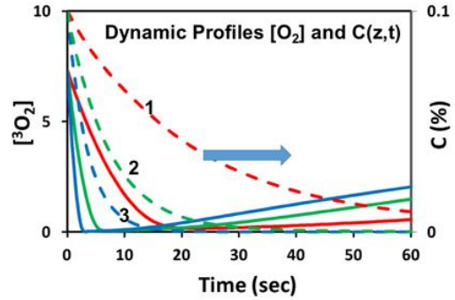
Fig. 4. The dynamic profiles of ground state oxygen (solid curves) and riboflavin (dashed curves) concentration (on surface, z=0 ), for intensity I_0 = (3,9,18) \text{ mW/cm}^2 (for curves in red, green, blue), for C_0=0.1\% , [O_0]=7.3 \text{ mg/L} , D=500 \mu\text{m} , D'=200 \mu\text{m} , and oxygen supply rate P_0=0.05 \text{ (1/s)}
