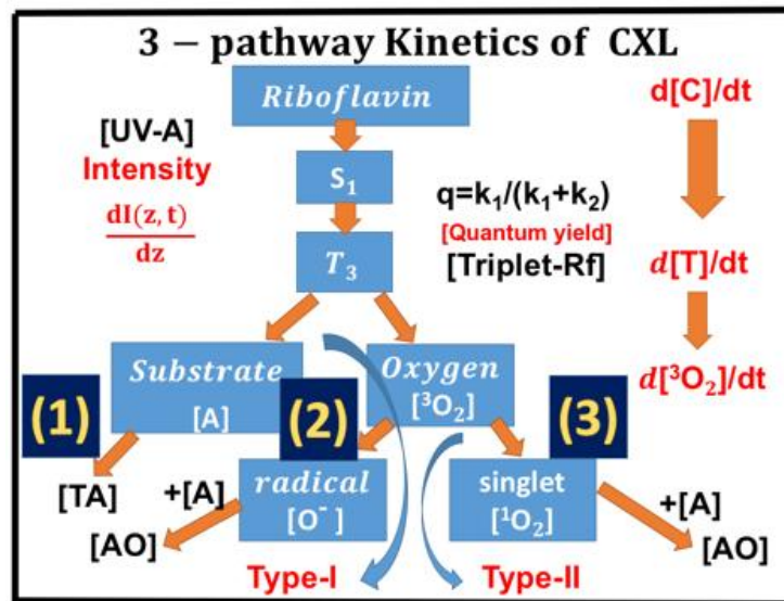
Fig. 2. The kinetics of CXL, where [ S_0 ], [ S_1 ] and [ T_3 ] are the ground state, singlet excited state, and triplet excited state of RF molecules. Three pathways are shown for both type-I and type-II process. Ground state oxygen may couple to T_3 to form either singlet oxygen [ O^* ], or other reactive radicals [ O^- ]. In type-I pathway, T_3 can interact directly with the collagen substrate (A); or with the oxygen ( O_2 ) to generate a superoxide anion ( O^- ); in type-II pathway, T_3 interacts with the ground oxygen ( O_2 ) to form a singlet oxygen ( O^* ) [13]
