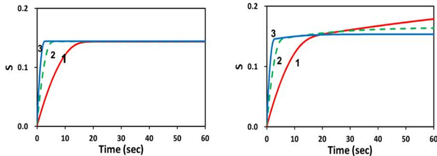
Fig. 5. The S-function profiles for Type-II ( S_2 ) associate to Fig. 4, but for P_0=0 (left figure) and P_0=0.05 (right figure)
