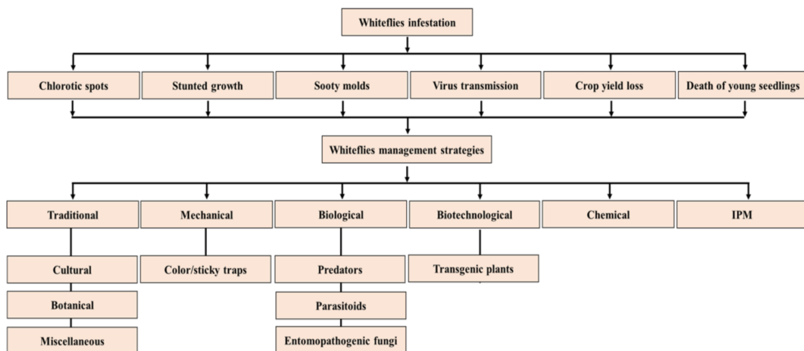
Fig. 2. A schematic representation of the available whitefly management (WFM) strategies (Source: https://www.mdpi.com/ )
