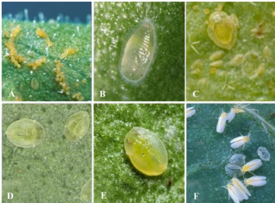
Fig. 1. The whitefly life cycle. (A) Oval-shaped eggs attached to the leaf via a stalk-like structure for fluid uptake, (B) the 1 st instar nymph, (C) 2 nd , 3 rd , and 4 th instar nymphs, (D) red-eyed 4 th instar nymph, (E) pharate adult stage or pupal stage, (F) emergence of adult whiteflies after metamorphosis leaving the transparent shells
