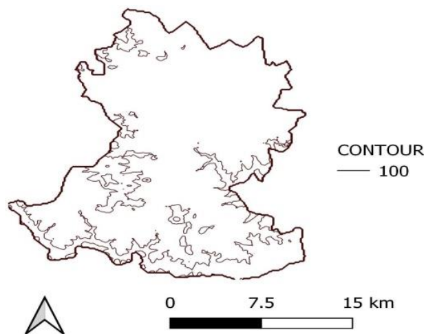
Fig. 6. Contour Map
